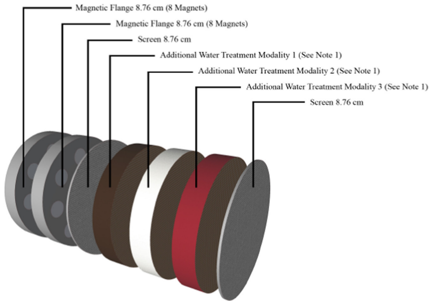
Fig. 2. Cross section of the Wellpure Water Treatment System. (Note 1 – These additional treatment modalities are not researched in this study).
