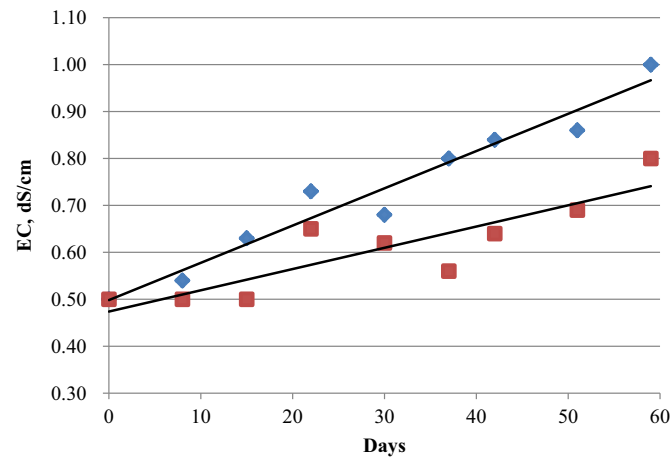
Fig. 3. EC accumulation over time - depth of 0–30 cm.
