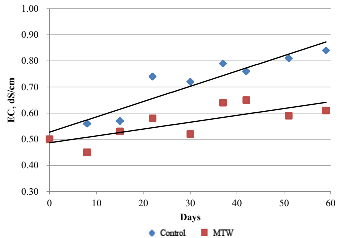
Fig. 4. EC accumulation over time - depth of 60 cm.
