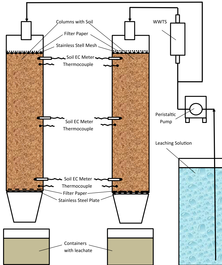
Fig. 1. Schematic diagram of soil column and flow chart (WSWT – Wellpure water treatment system).
